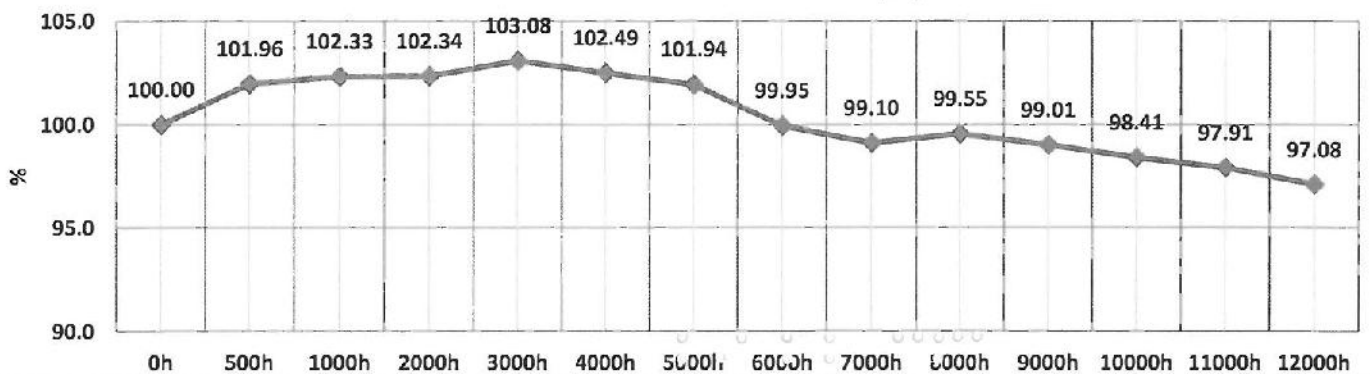
Lumen Maintenance (%)
